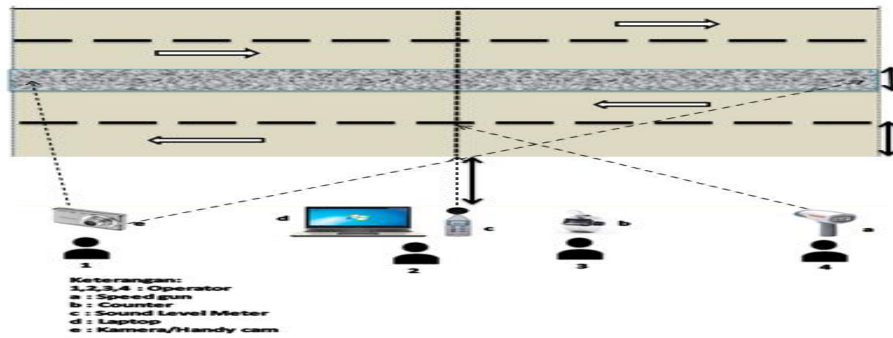
Figure 1. Measurement Method
